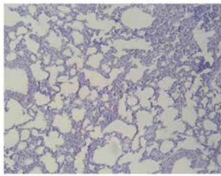
Normal
