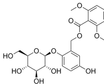
CURCULIGOSIDE-STRUCTURE
