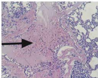
Metastatic control
